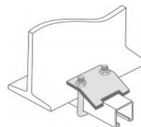
Our Ref: BF048 Unistrut Ref: P2785
