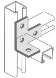
Our Ref: BF029 Unistrut Ref: P1035
