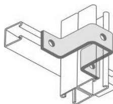
Our Ref: BF011 Unistrut Ref: P1737
