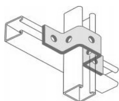
Our Ref: BF010 Unistrut Ref: P1047
