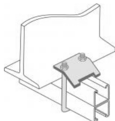
Our Ref: BF049 Unistrut Ref: P2786
