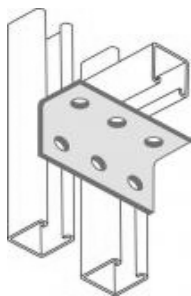
Our Ref: BF041 Unistrut Ref: P1060-S1
