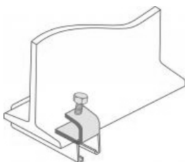
Our Ref: BF046 Unistrut Ref: P1272
